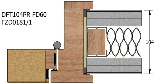
2-part Rebated Doorframe FD60
