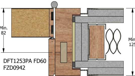
3-part Panel Stop Doorframe FD60
