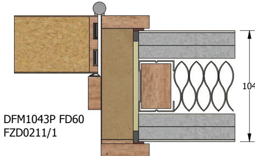
3-part MDF Doorframe FD60
