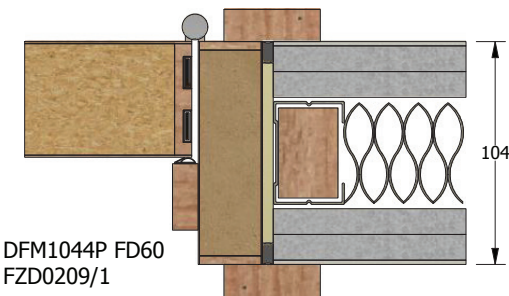
4-part MDF Doorframe FD60
