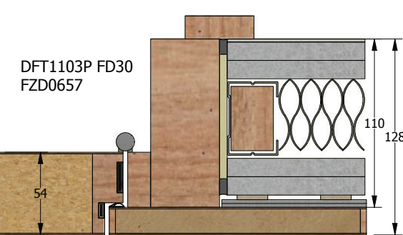
3-part Panel Stop Doorframe FD30
