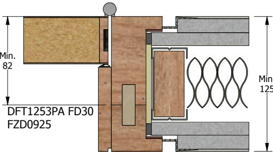
3-part Panel Stop Doorframe FD30
