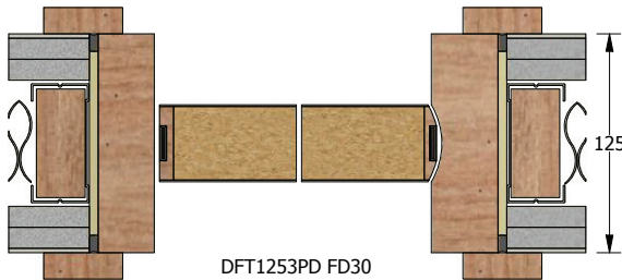
DFT1253PD FD30 FZD0172
