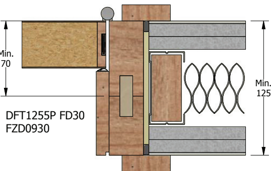
5-part Split Doorframe FD30
