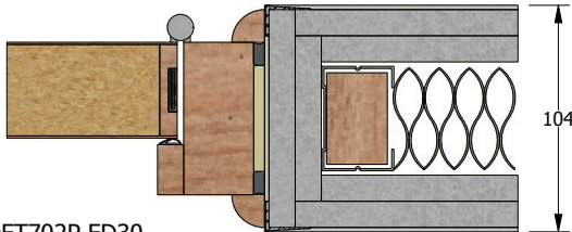
DFT702P FD30 FZD0173
