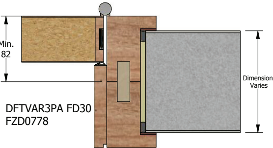
5-part Split Doorframe FD30
