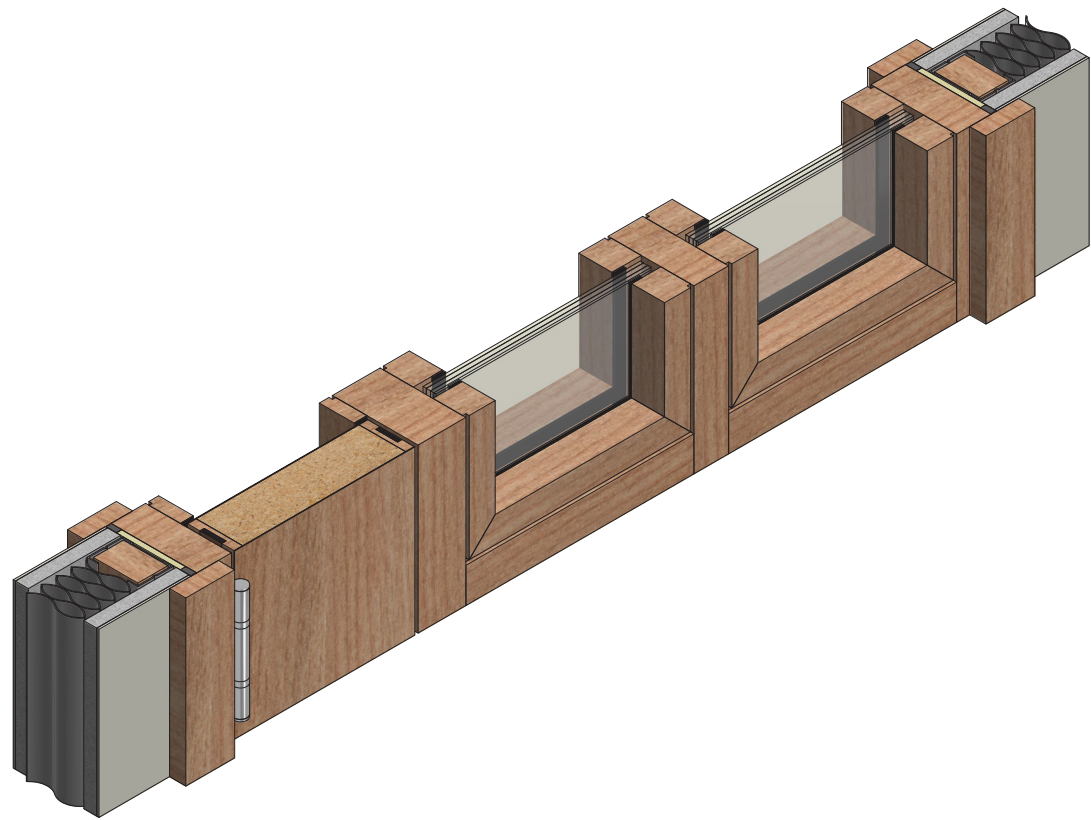
Isometric Timber/ Steel Stud FD30
