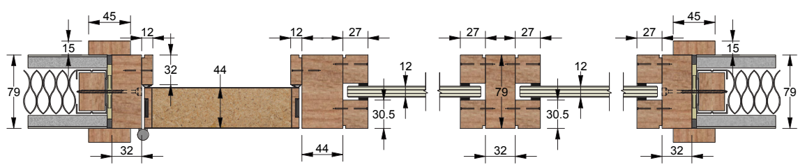
Detail Timber/ Steel Stud FD30
