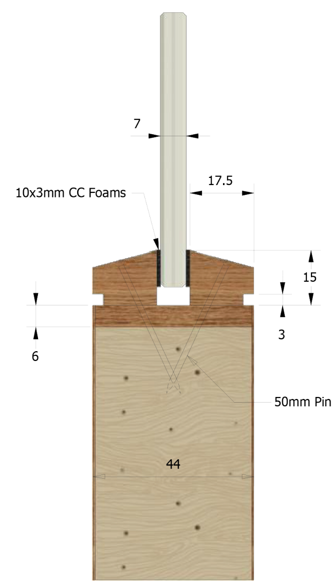
SPLAYED
