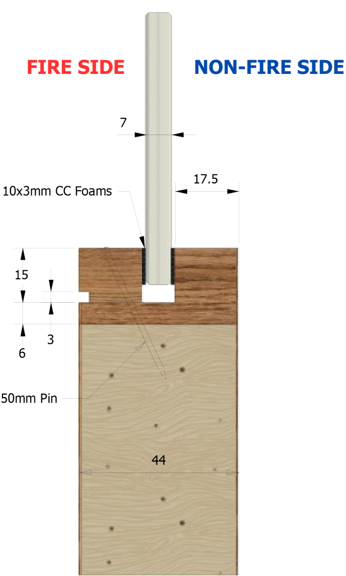
CONCEALED
