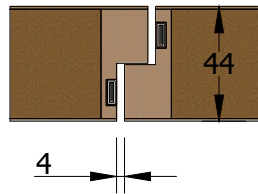
Detail D
