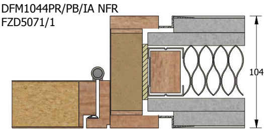
4-part Rebated Shadow-gap MDF Doorframe NFR
