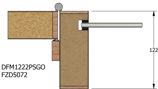
2-part MDF Doorframe SGO NFR
