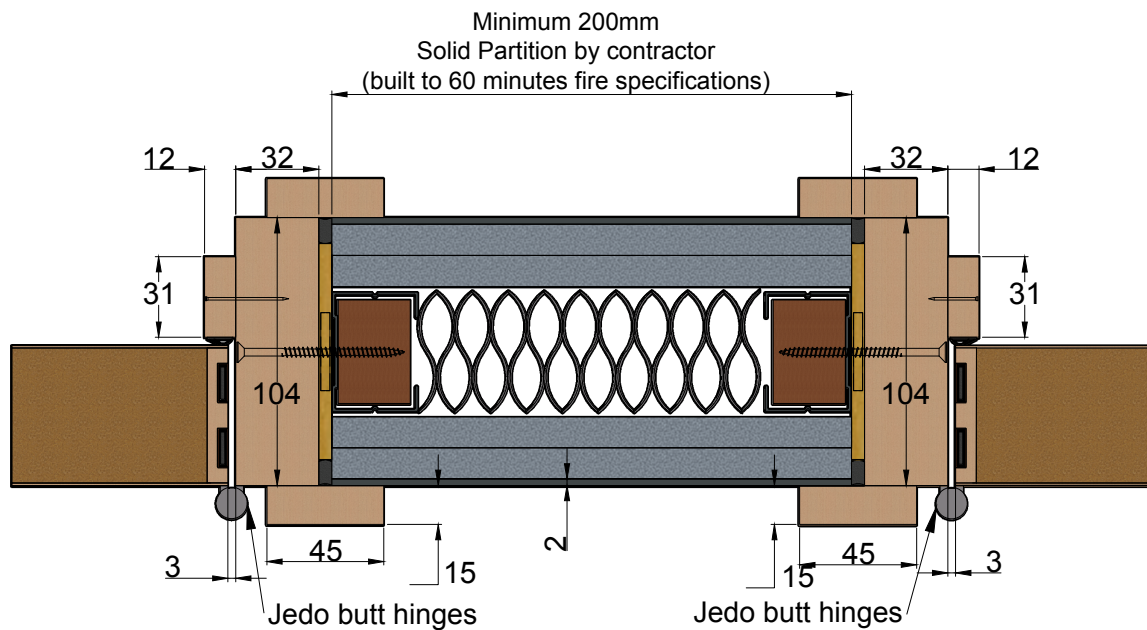
Detail D
