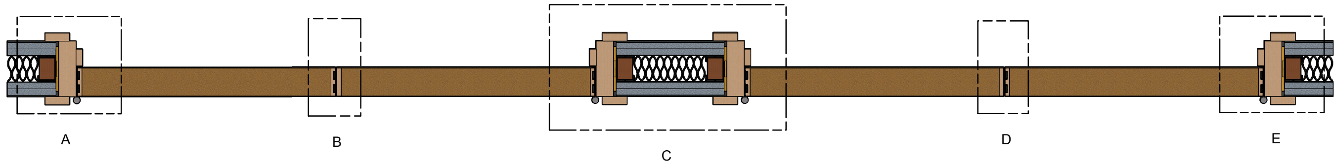
Plan Detail
