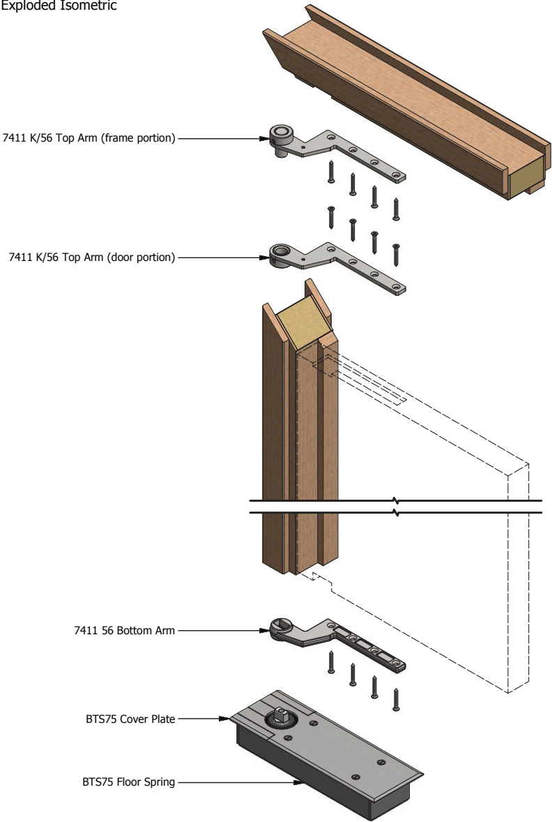
Exploded Isometric
