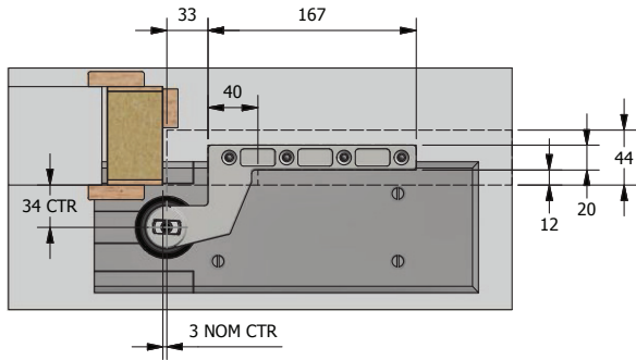
Plan Section (Door Base)
