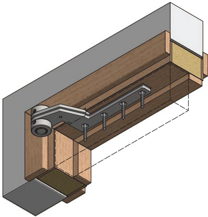
Isometric - Door Head
