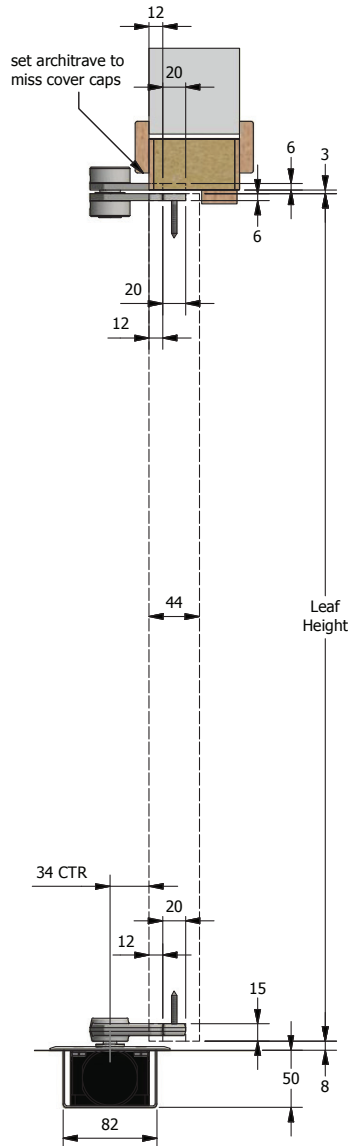
Vertical Section
