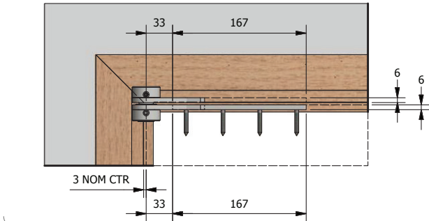
Plan Section (Door Base)
