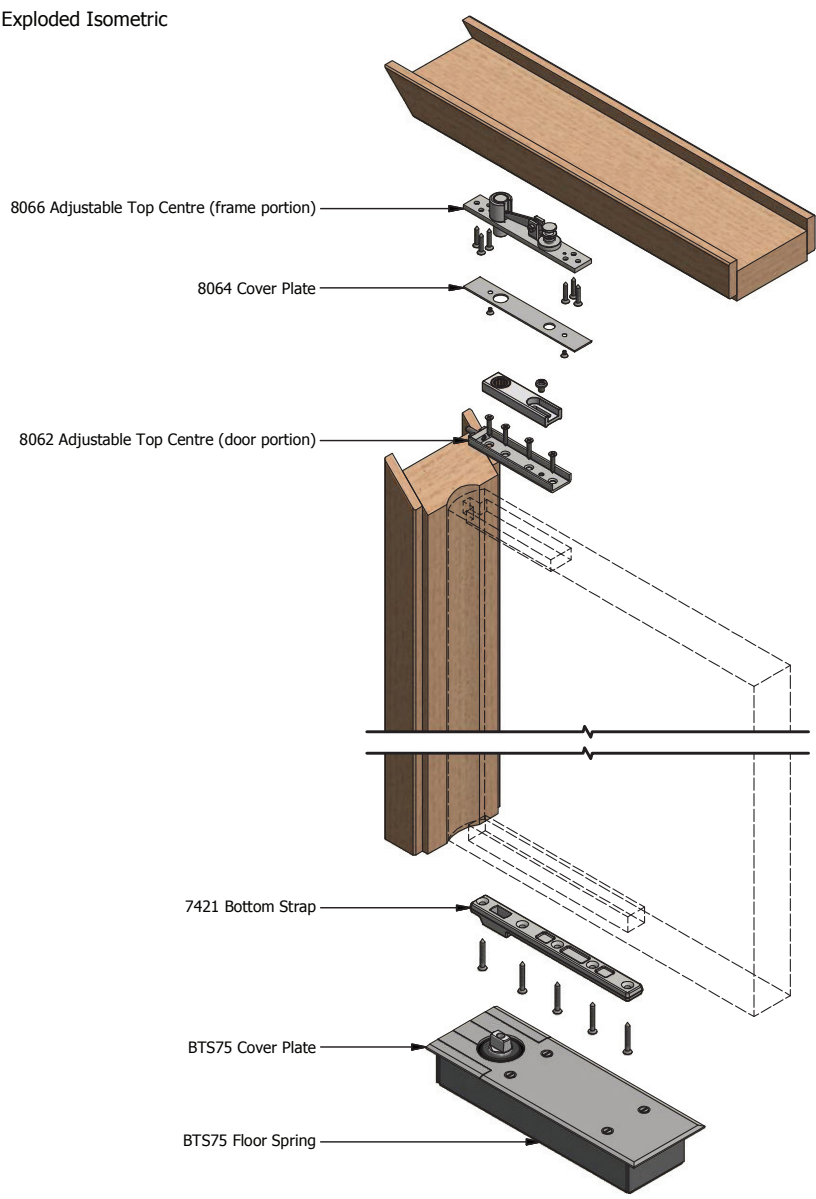
Exploded Isometric
