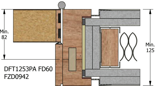
3-part Panel Stop Doorframe FD60
