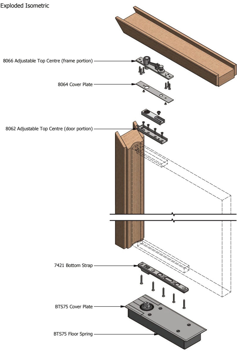
Exploded Isometric
