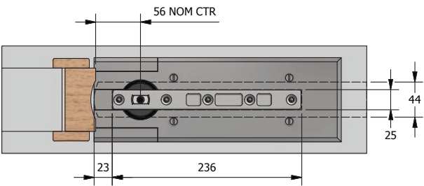
Plan Section (Door Base)
