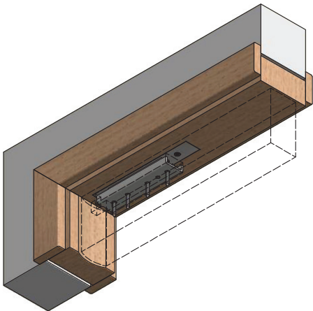
Isometric - Door Head
