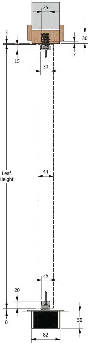
Vertical Section
