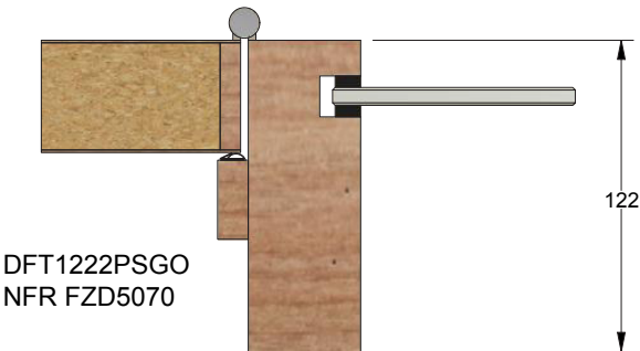
2-part Timber Doorframe SGO NFR
