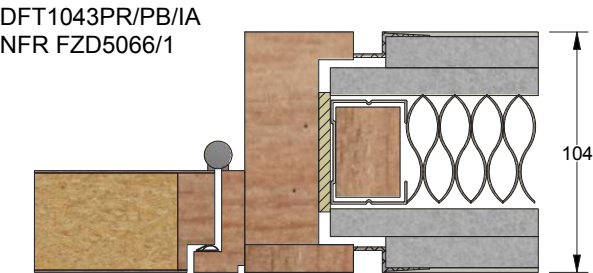
3-part Rebated Shadow-gap Doorframe NFR
