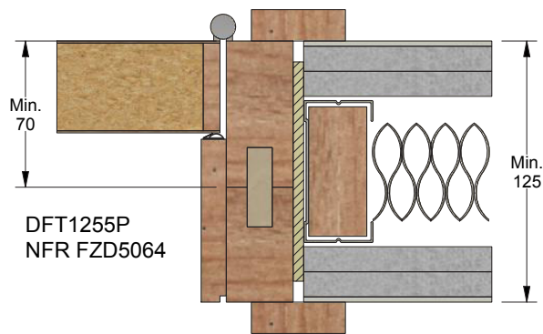
5-part Split Doorframe NFR
