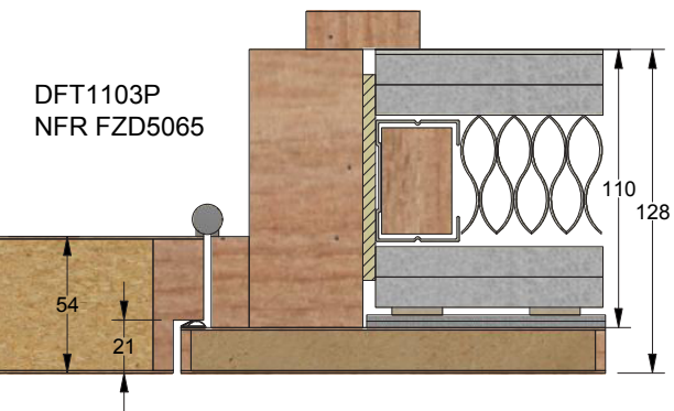
3-part Panel Stop Doorframe NFR
