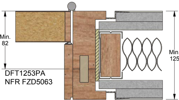
3-part Panel Stop Doorframe NFR
