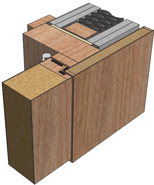
Isometric
