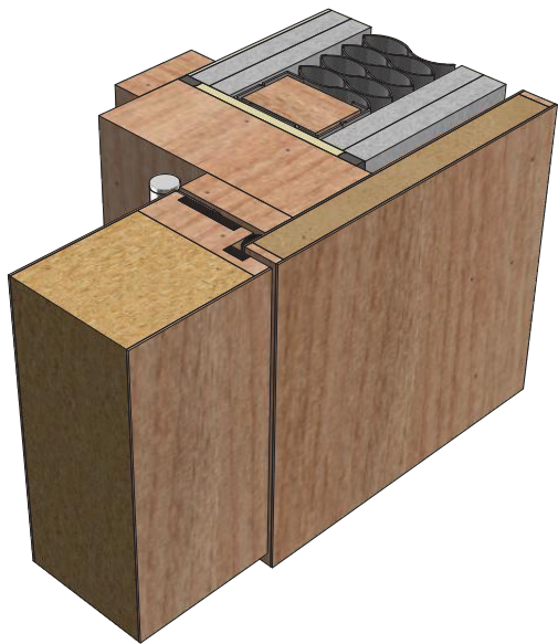
Isometric
