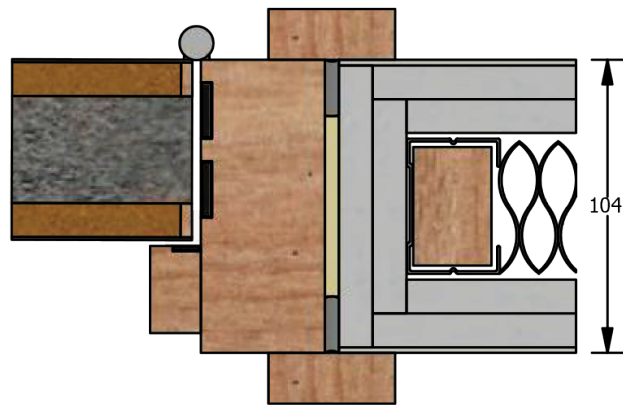
4-part Timber Doorframe FD120 (FCH)
