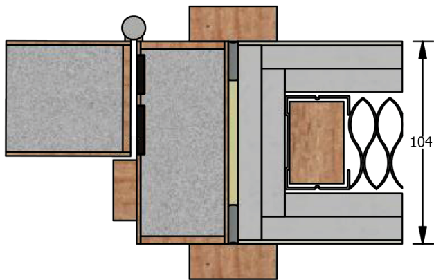
4-part Composite Doorframe FD120 (FCW)
