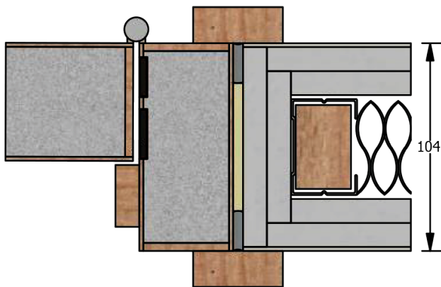
4-part Composite Doorframe FD90 (FCW)
