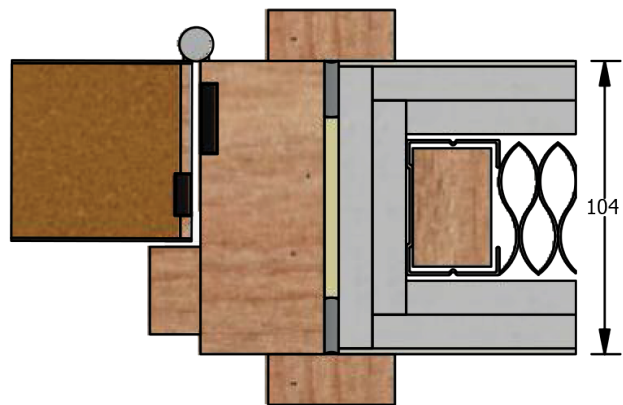
4-part Timber Doorframe FD90 (FCH)
