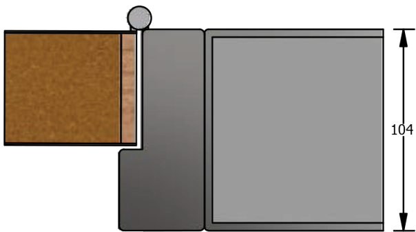
Generic Steel Doorframe FD90 (FCH)
