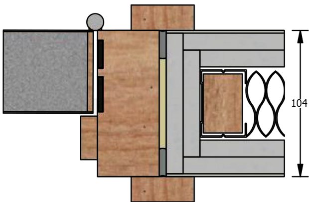
4-part Timber Doorframe FD90 (FCW)
