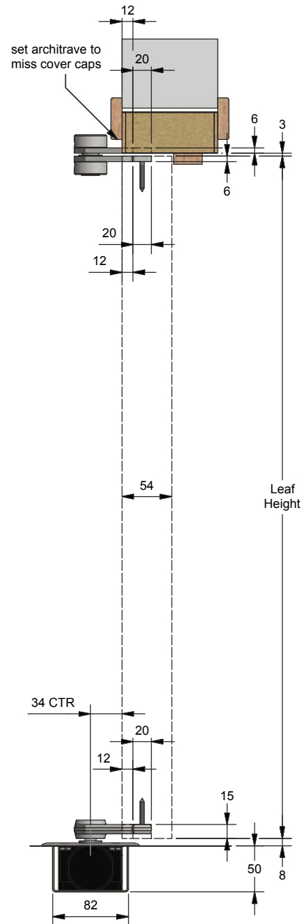
Vertical Section
