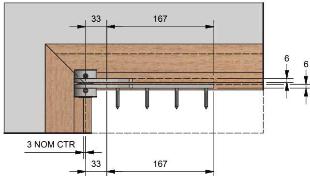
Plan Section (Door Base)
