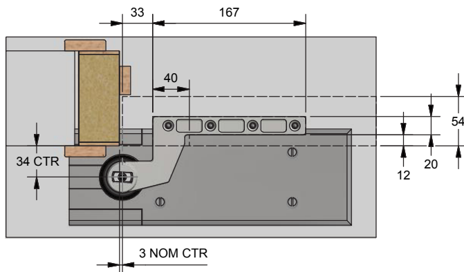
Plan Section (Door Base)
