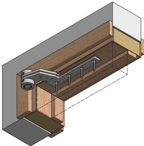
Isometric - Door Head
