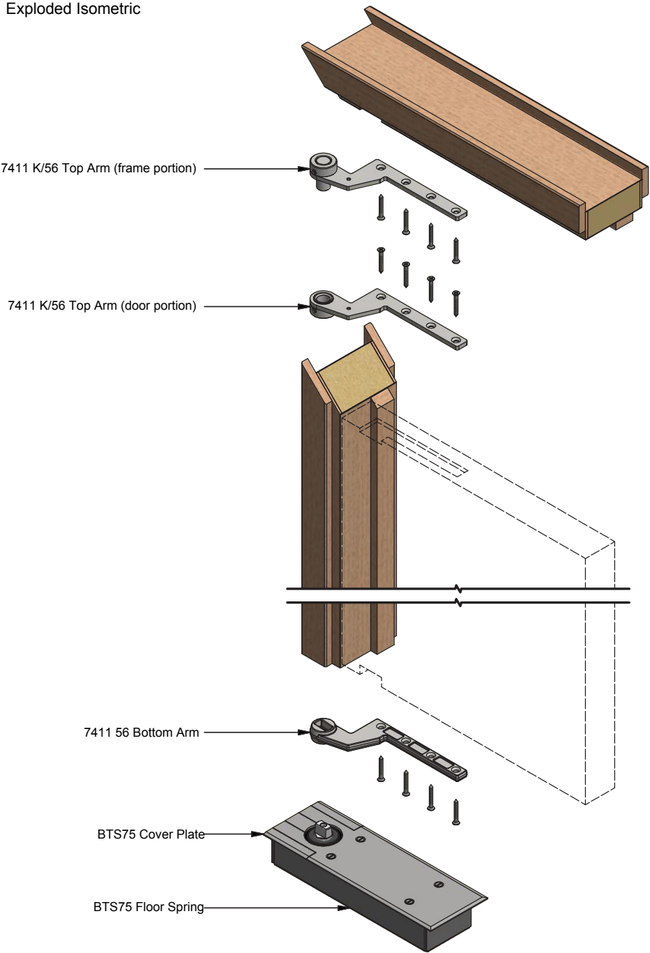
Exploded Isometric
